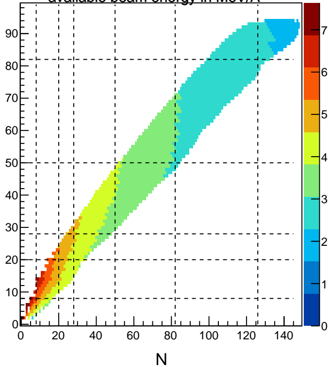
ReA3 - Contours depict maximum available beam energy in MeV/A
