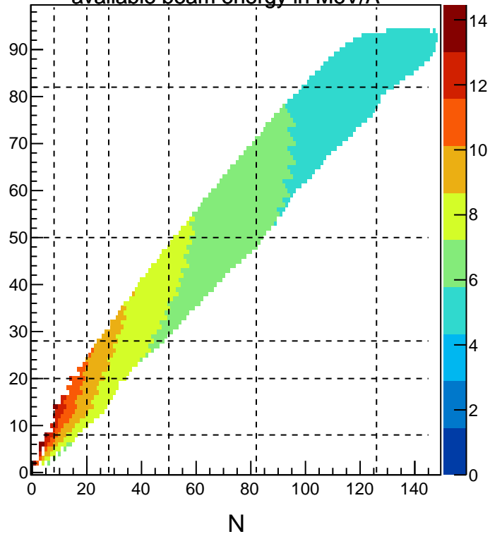
ReA6 - Contours depict maximum available beam energy in MeV/A
