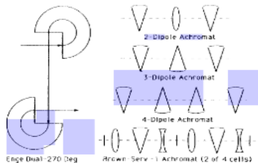
Figure 1. First-order achromats.
