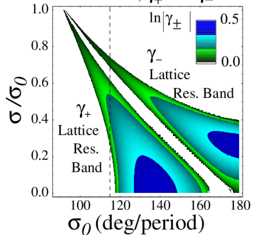
Breathing and Quadrupole Mode Growth Factors, \gamma_+ and \gamma_-
