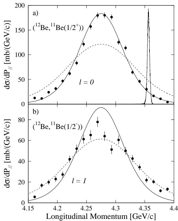
FIG. 2. Laboratory frame longitudinal momentum distributions for {}^{11}\text{Be} residues in the ground (a) and excited (b) states. The solid (dashed) curves are calculated for l = 0 (1) neutron removal. The narrow line in (a) illustrates the line profile of the spectrograph.
