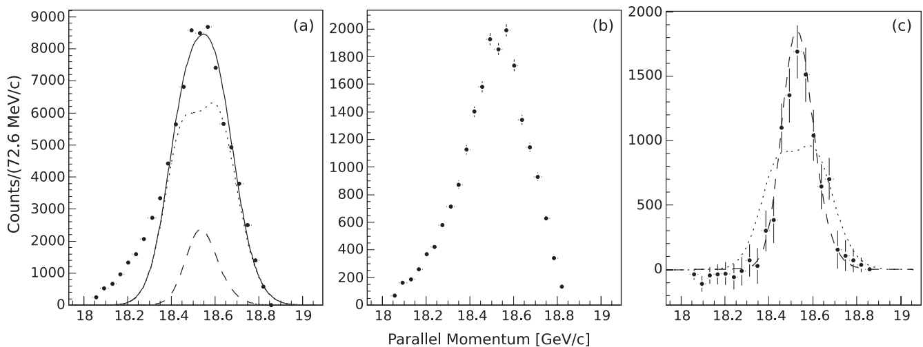
FIG. 2. (a) Inclusive, (b) \gamma -gated, and (c) ground-state parallel momentum distributions of ^{44}\text{Cl} particles produced in one-neutron knockout from ^{45}\text{Cl} . The dashed (dotted) curves are theoretical distributions for l = 1 ( l = 3 ) neutron removal. The solid curve in panel (a) is the fit described in the text.
