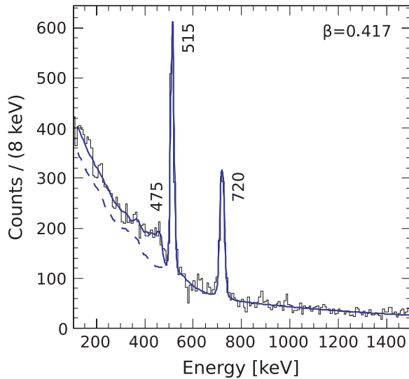
FIG. 1. (Color online) Spectrum of \gamma rays measured in coincidence with recoiling ^{44}\text{Cl} particles. The solid curve is the GEANT4 fit described in the text. The dashed curve is the fit without the 475-keV \gamma ray.
