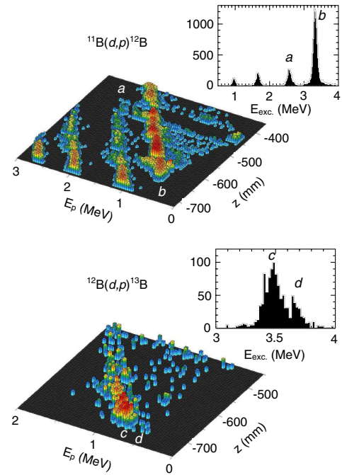
FIG. 2 (color online). Raw data from ^{11}\text{B}(d,p)^{12}\text{B} (top) and ^{12}\text{B}(d,p)^{13}\text{B} (bottom). The three-dimensional plots (with units displayed logarithmically) in the E_p vs z plane show ridges that correspond to different excited states of the final nucleus. The insets show the projection of the data onto excitation energy in the final nucleus. The states labeled a and b in the upper image correspond to the 2.62- and 3.39-MeV states of ^{12}\text{B} , while in the lower one the labels c and d are the 3.48/3.68-MeV doublet studied in ^{13}\text{B} . The range in z corresponds to angles of \sim 10^\circ\text{--}30^\circ in the center of mass.
