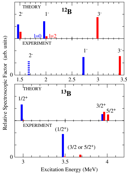
FIG. 4 (color online). Energies and spectroscopic factors for \ell = 0 and 2 ( d, p ) transitions from theory and experiment, with ^{12}\text{B} on top and ^{13}\text{B} on bottom. Solid bars are experimental values from the present measurement, the dashed bar is from other work. Only relative values of spectroscopic factors are meaningful within each plot, and the two colors denote the two \ell values as indicated. The small \ell = 2 component shown as the experimental result for the 3.48-MeV state is a limit.
