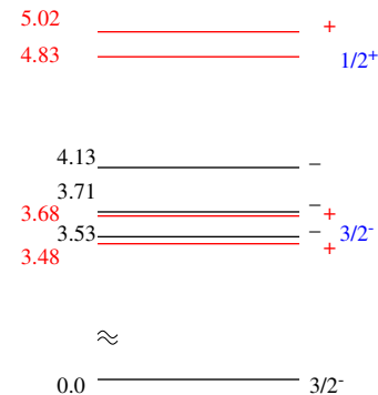
FIG. 1 (color online). The observed levels in ^{13}\text{B} , up to \sim 5 -MeV excitation, from various sources. The negative- and positive-parity states of Ref. [1] are indicated [black and light gray (red)] with a “-” or “+” on the right-hand margin. The recent spin assignments [3,4] are in dark gray (blue) on the right-hand side.
