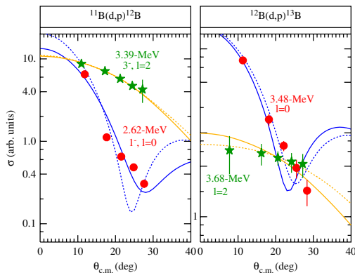
FIG. 3 (color online). The left-hand figure shows angular distributions for the ^{11}\text{B}(d,p)^{12}\text{B} reaction measured with HELIOS for two states known to be populated with \ell = 0 and 2. The normalization procedure is described in the text and this plot used the \ell = 2 transition for reference. The solid stars (green) are the HELIOS data for the \ell = 2 transition to the 3.39-MeV state, used as a basis of normalization, and the solid dots (red) are the \ell = 0 , 2.62-MeV state. The solid lines and the dashed lines are DWBA calculations with two different sets of parameters. On the right, the data for the ^{12}\text{B}(d,p)^{13}\text{B} doublet at 3.48 and 3.68 MeV are shown with the same normalization. The conventions on the symbols and curves are the same as on the left-hand side. Angles, \theta_{\text{c.m.}} , are in the center of mass.
