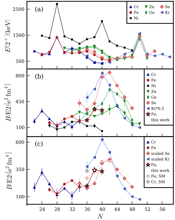
FIG. 2 (color online). (a) Energies E(2^+) and (b) B(E2; 2^+ \rightarrow 0^+) values for even-even nuclei with Z = 24 –36 and N = 22 –58. The stars indicate the present data of ^{62,64,66}\text{Fe} . The B(E2) data of Kr in (b) are divided by 2. In (c), the B(E2) data of the Fe and Cr isotopes are compared to the scaled B(E2) values for the Se and Kr isotopes, respectively, as well as the shell-model predictions (SM) for ^{62,64,66,68}\text{Fe} and ^{60}\text{Cr} isotopes.
