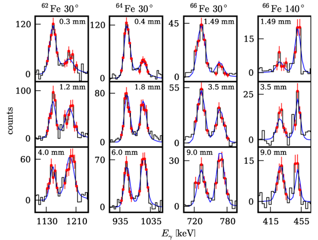
FIG. 1 (color online). Typical results from the \gamma -ray line-shape fits to the data for the 2^+ \rightarrow 0^+ transitions in ^{62,64,66}\text{Fe} .
