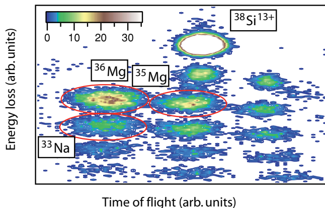
FIG. 1. (Color online) Identification spectrum for the reaction residues produced in {}^9\text{Be}({}^{38}\text{Si}, A Z)X at 83 MeV/u midtarget energy. All reaction residues can be unambiguously identified by plotting the energy loss measured in the S800 ionization chamber vs the ion's time of flight. The magnetic rigidity of the S800 spectrograph was set to center {}^{36}\text{Mg} in the focal plane (see Ref. [13]). The H-like charge state of the projectile beam, produced by electron pickup of the originally fully stripped {}^{38}\text{Si} passing through the reaction target, is the most intense constituent of the reacted beam.
