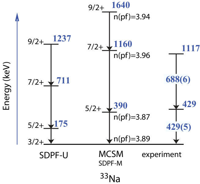
FIG. 5. (Color online) Level schemes of ^{33}\text{Na} as calculated in the shell model (left) compared to the measured \gamma -ray transitions. Assuming that the observed 429- and 688-keV transitions are in coincidence, the experimental level scheme agrees very well with the MCSM using the SDPF-M effective interaction.
