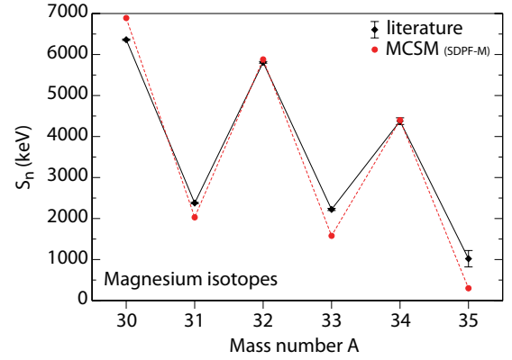
FIG. 4. (Color online) Neutron separation energies S_n for neutron-rich magnesium isotopes from the literature ( A = 30-33 taken from Ref. [32]; A = 34, 35 based on the mass excess reported in Ref. [31]) compared to the MCSM (SDPF-M) calculations. The overestimated odd-even staggering supports the assumption that pairing effects are overestimated, leading to an underestimation of S_n for the odd- A isotopes by several hundred keV.
