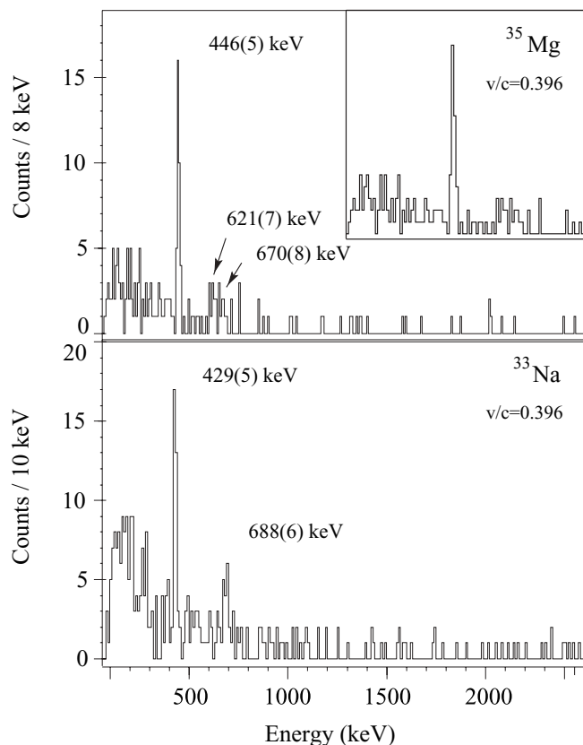
FIG. 2. (top) Doppler-reconstructed \gamma -ray spectrum in coincidence with {}^{35}\text{Mg} reaction residues. (bottom) Gamma-ray spectrum in coincidence with {}^{33}\text{Na} .
