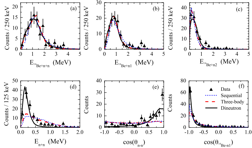
FIG. 2 (color online). (a) Three-body decay energy from the reconstruction of ^{14}\text{Be} + n + n . (b),(c) Two-body decay energy of ^{14}\text{Be} + n , where (b) corresponds to the highest decay energy and (c) to the lowest. (d) Two-body relative energy of the two neutrons. (e) Opening angle \theta_{n-n} between the two neutrons in the center-of-mass frame of ^{16}\text{Be} . (f) Opening angle ( \theta_{^{14}\text{Be}-n1} ) between the ^{14}\text{Be} fragment and the first neutron in the center-of-mass frame of ^{16}\text{Be} . In all figures, the experimental data are shown in black triangles, the sequential emission in dotted lines, the three-body decay in dashed lines, and the dineutron decay in solid lines.
