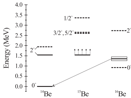
FIG. 1. Level and decay scheme for neutron-rich isotopes of beryllium. The solid lines correspond to experimental data from [17,15], and the present Letter, while the dashed lines represent shell model calculations in the s - p - sd - pf model space using the WBP interaction [18].
