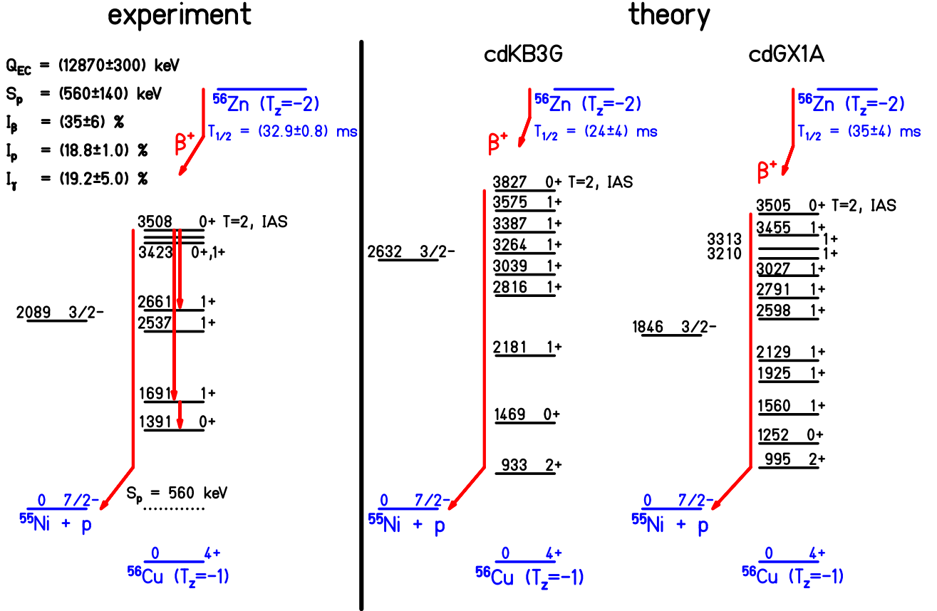
FIG. 1. Experimental and theoretical partial decay schemes of ^{56}\text{Zn} . The experimental Q_{\text{EC}} value and the proton separation energy S_p are from AME2003 [5]. I_\beta is the theoretical \beta feeding of the IAS and I_p and I_\gamma are the experimental proton- and \gamma -emission branching ratios from the IAS. The theoretical calculations have been performed with two different effective interactions, cdKB3G and cdGX1A.
