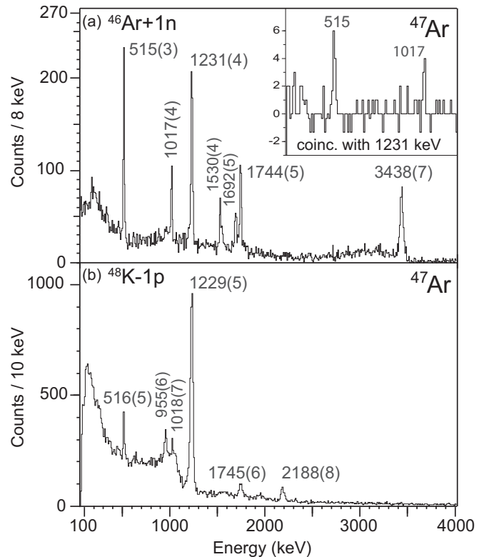
FIG. 2. Event-by-event Doppler-reconstructed \gamma -ray spectra of ^{47}\text{Ar} : (a) as detected with GREYINA following ^{12}\text{C}(^{46}\text{Ar}, ^{47}\text{Ar} + \gamma)X one-neutron pickup ( v/c = 0.337 ) using nearest-neighbor addback, and (b) one-proton removal ^9\text{Be}(^{48}\text{K}, ^{47}\text{Ar} + \gamma)X with \gamma -ray spectroscopy using SeGA ( v/c = 0.4 ). The inset to panel (a) shows a coincidence spectrum with a software gate applied on the 1231 keV line indicating that the 515, 1016, and 1231 keV transitions are in coincidence.
