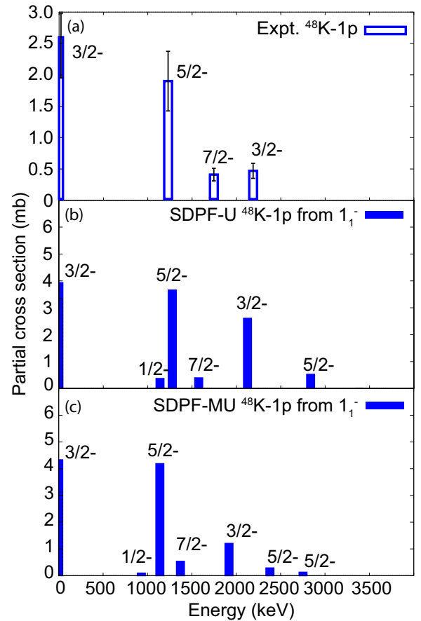
FIG. 5. One-proton-removal partial cross sections to ^{47}\text{Ar} final states (a) as measured in the experiment, and as calculated following Sec. II with (b) SDPF-U and (c) SDPF-MU shell-model spectroscopic factors. The shell-model calculations use the wave function of the lowest-lying 1^- state, although this is not the ground state in either shell-model calculation. The J^\pi = 1^- spin assignment was determined from laser spectroscopy [29].
