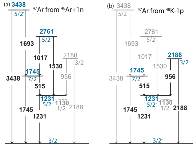
FIG. 3. Level scheme of {}^{47}\text{Ar} as observed in (a) one-neutron pickup and (b) one-proton removal. Levels and transitions indicated in black were observed to be populated with the respective reaction, levels and transitions marked in gray are known but were not observed in the respective reaction. The complementarity of the two reactions is apparent. Only the 1130 keV 1/2^- state [18] could not be accessed in the presented measurements.
