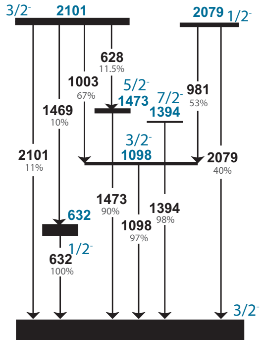
FIG. 7. SDPF-U shell-model level scheme of ^{45}\text{S} . The widths of the lines representing energy levels are proportional to the calculated partial cross section for the ^9\text{Be}(^{46}\text{Cl}, ^{45}\text{S})X one-proton-removal reaction, taking the wave function of the lowest 1^- state as the ground state of ^{46}\text{Cl} (see text and Table III). Only states predicted to be populated with more than 0.2 mb cross section are shown and only transitions with a branching ratio of 10% or higher are drawn.
