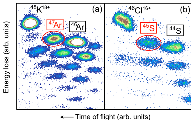
FIG. 1. Particle identification spectra for the one-proton-removal reactions to (a) ^{47}\text{Ar} and (b) ^{45}\text{S} used to determine the inclusive cross sections. The most intense structure in each spectrum is the hydrogen-like charge state of the projectile beam.
