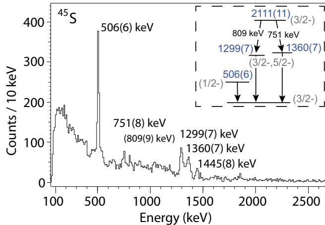
FIG. 6. Event-by-event Doppler-reconstructed \gamma -ray spectrum of ^{45}\text{S} following population of the nucleus in the ^9\text{Be}(^{46}\text{Cl}, ^{45}\text{S} + \gamma)X one-proton-removal reaction ( v/c = 0.393 ). The inset shows a tentative level scheme based on energy sums, intensity arguments, and comparison with shell-model calculations (see text).
