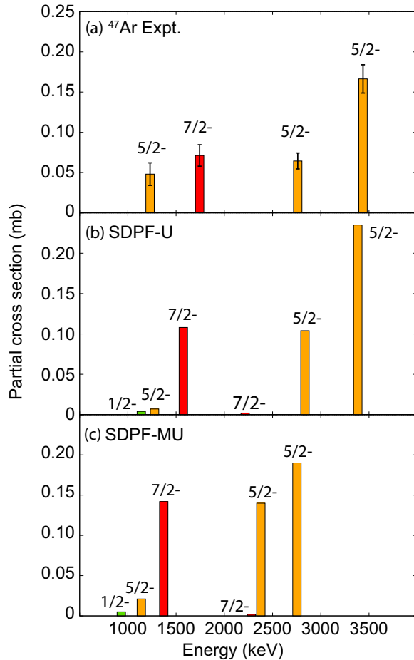
FIG. 4. One-neutron pickup partial cross sections to excited final states (a) as measured in the experiment, and as calculated following Sec. II, with the (b) SDPF-U and (c) SDPF-MU SM spectroscopic factors.
