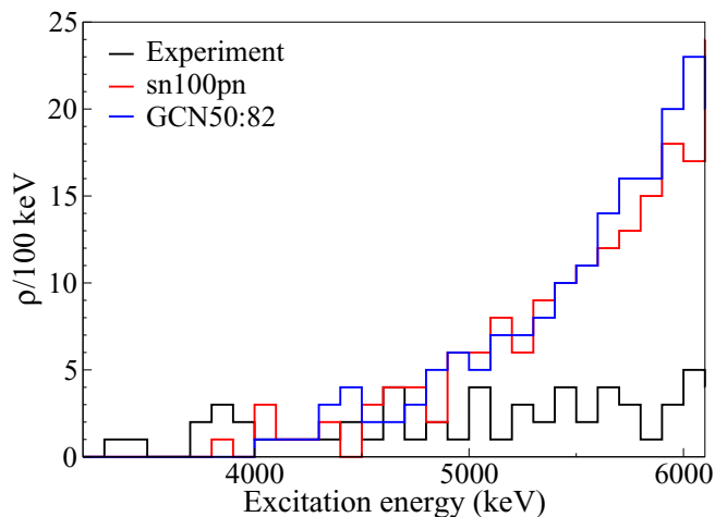
FIG. 15. A similar comparison as Fig. 14, but for higher-lying 1^- states. Here, we include all the J = 1 states reported in the literature [59], as they were mostly identified via inelastic photon scattering which has high selectivity in populating 1^- levels.
