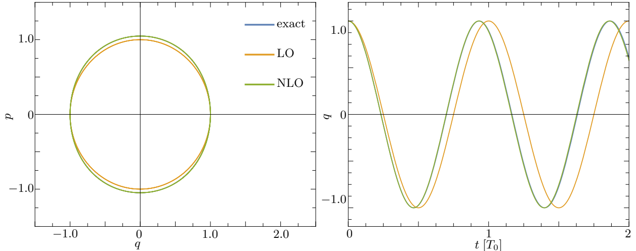
Figure 4: Poincaré-Lindstedt solutions for the Duffing oscillator with A = 1, \omega_0, \epsilon = 0.2 .
