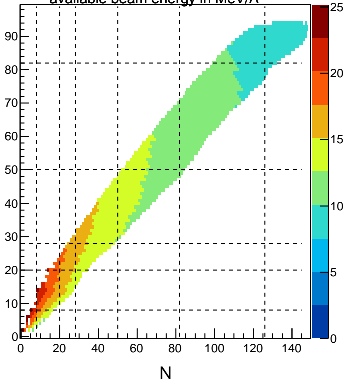
ReA12 - Contours depict maximum available beam energy in MeV/A
