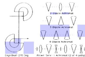
Figure 1. First-order achromats.
