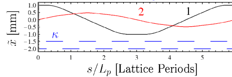
Simple harmonic oscillations modified with additional harmonics due to periodic focus
