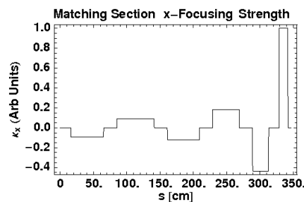
Example corresponds to High Current Experiment Matching Section (hard edge equivalent) at LBNL (2002)
