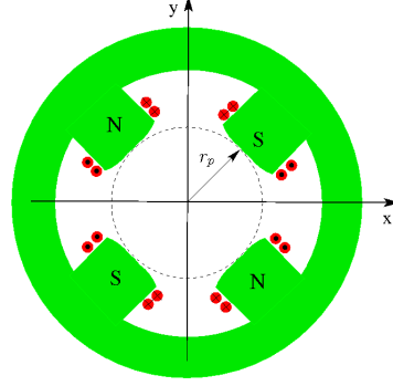
Shaped Iron Pole Sections (finite)
