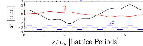
Simple harmonic oscillations more strongly modified due to periodic AG focus
