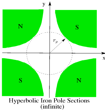
Ideal (infinite geometry)
