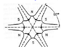
Sextupole (n=3)
