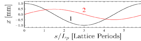
Simple Harmonic Oscillator
