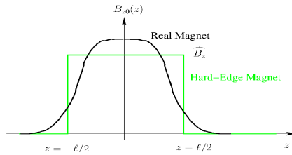
Hard-Edge and Real Magnets axially centered to compare
