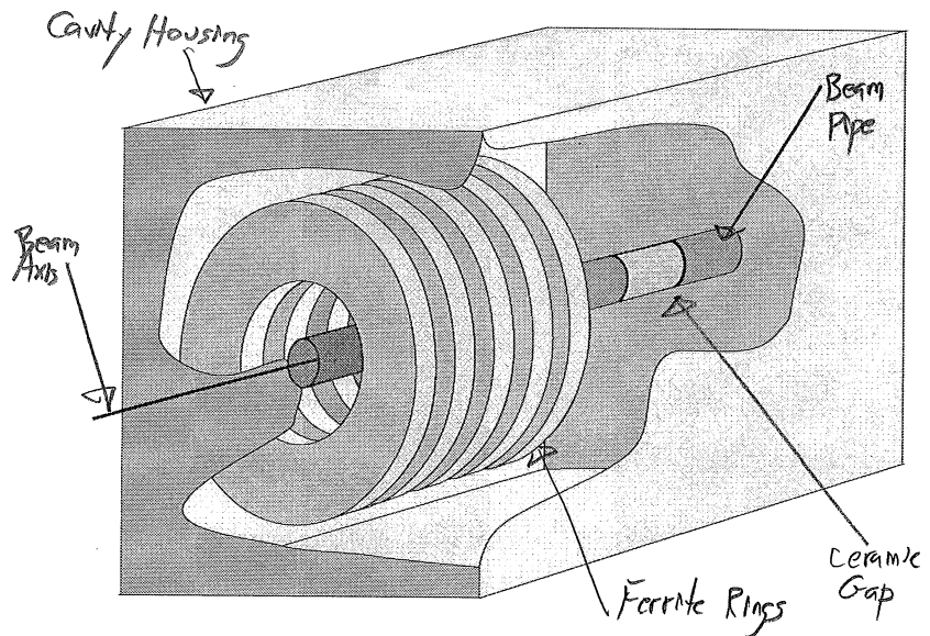
Fig. 2: Simplified 3D sketch of a ferrite-loaded cavity
