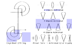
Figure 1. First-order achromats.
