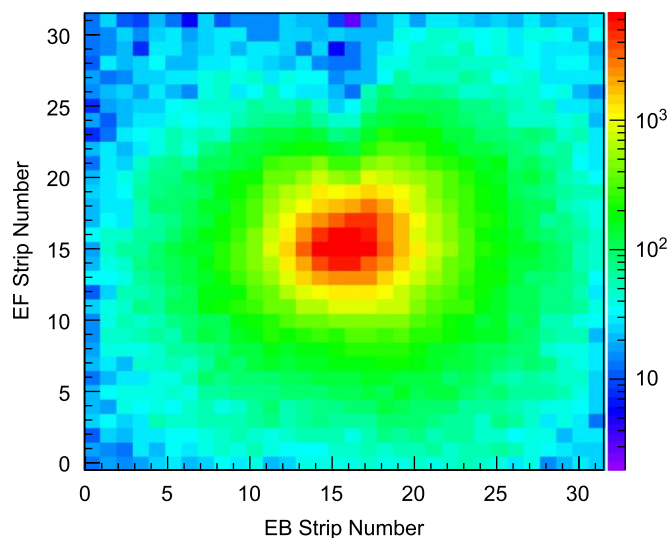
Fig. 15. The two-dimensional hit pattern from a pin source inserted between the two silicon detectors of a HiRA telescope.
