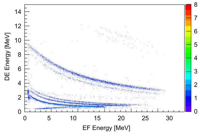
Fig. 18. A PID spectrum using both silicon detectors.
