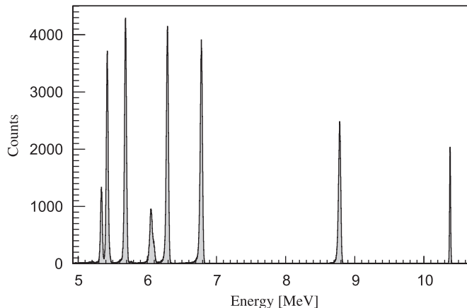
Fig. 8. A ^{228}\text{Th} spectrum with a pulser peak above 10 MeV for a single strip of a HiRA double-sided silicon strip-detector.
