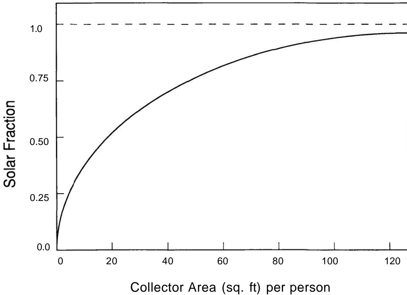
Figure E-4. Solar Fraction Versus Collector Area.
