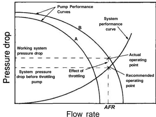
Figure 4-9. Typical Pump and System Operation Curves.
