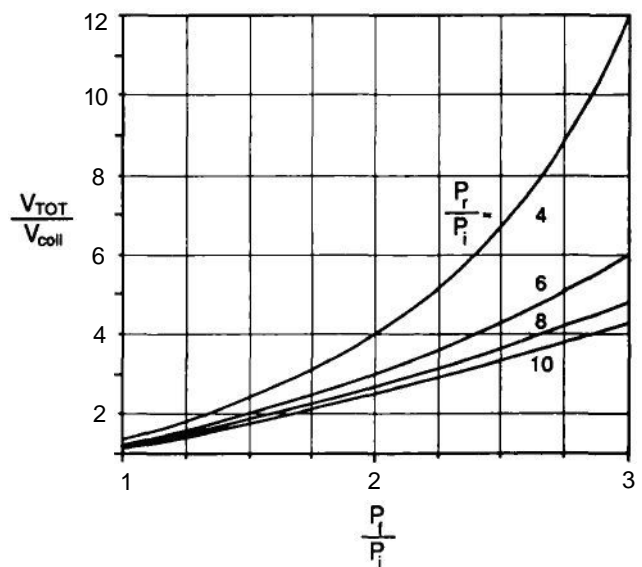
Figure 4-8. Calculation of Total Expansion Tank Volume as a Function of System Pressures and Acceptance Volume.
