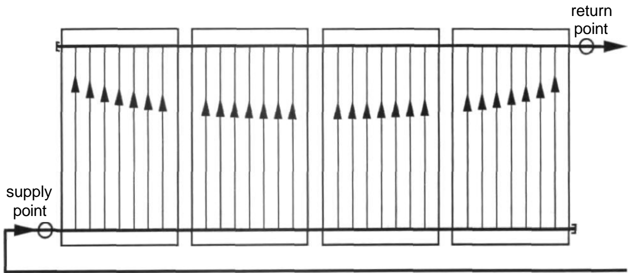
(a) Reverse - return bank piping
