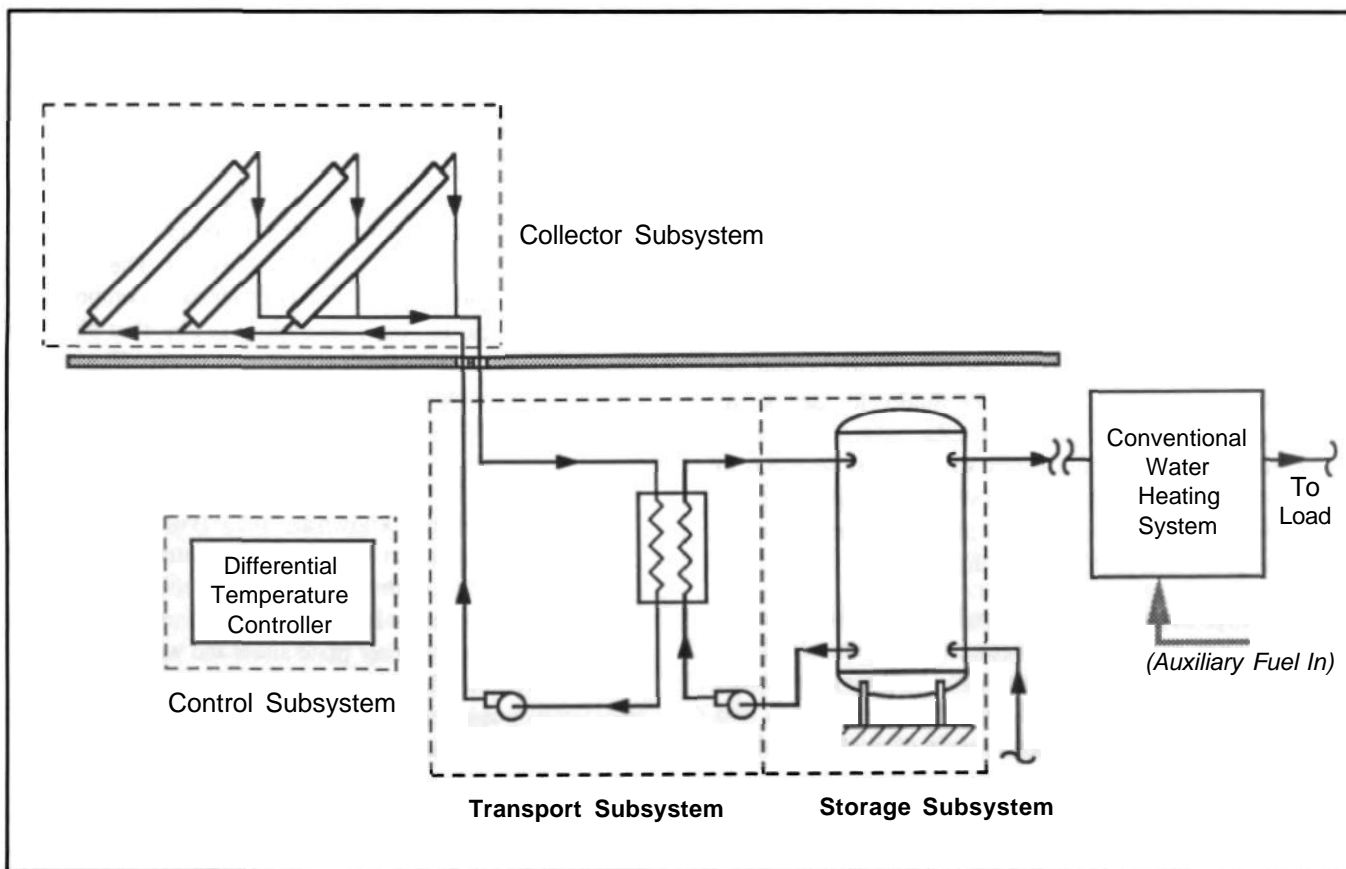
Figure E-1. A Typical Solar Thermal Energy System.
