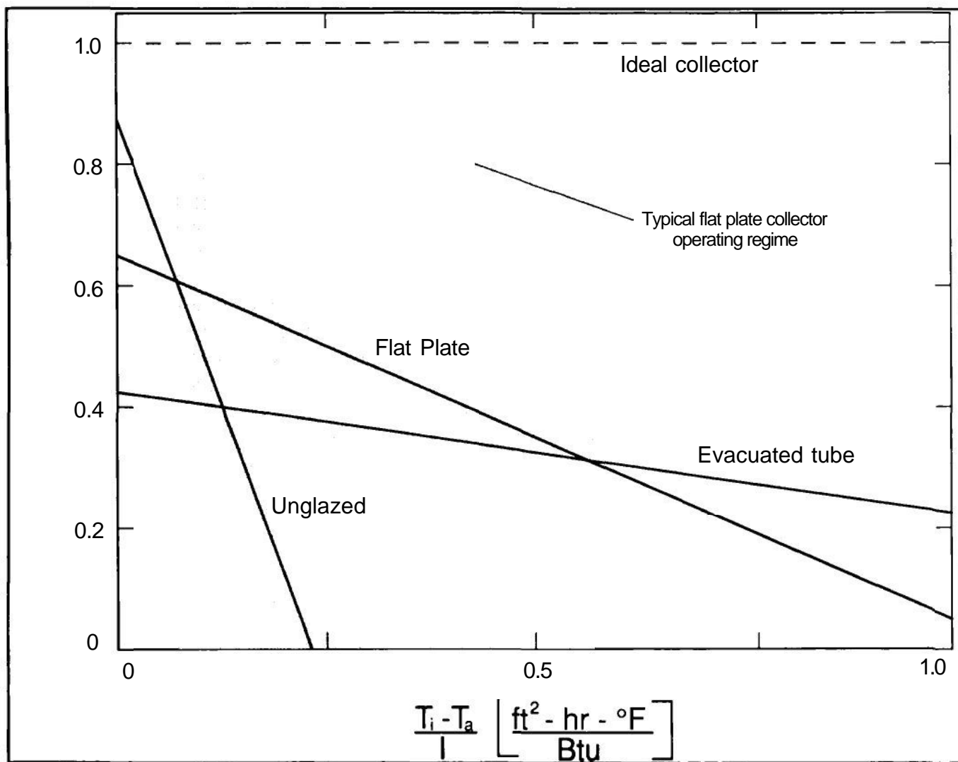
Figure E-3. Typical Solar Collector Efficiency Plots
