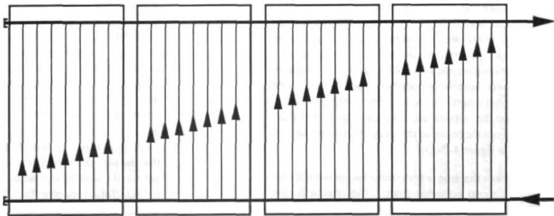
(b) Direct return bank piping (not allowed)
