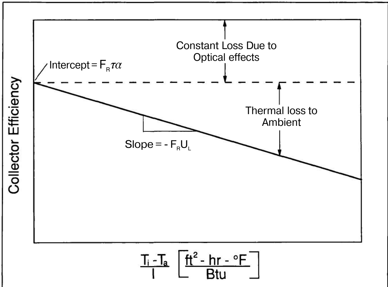
Figure E-2. Typical Collector Efficiency Curve.
