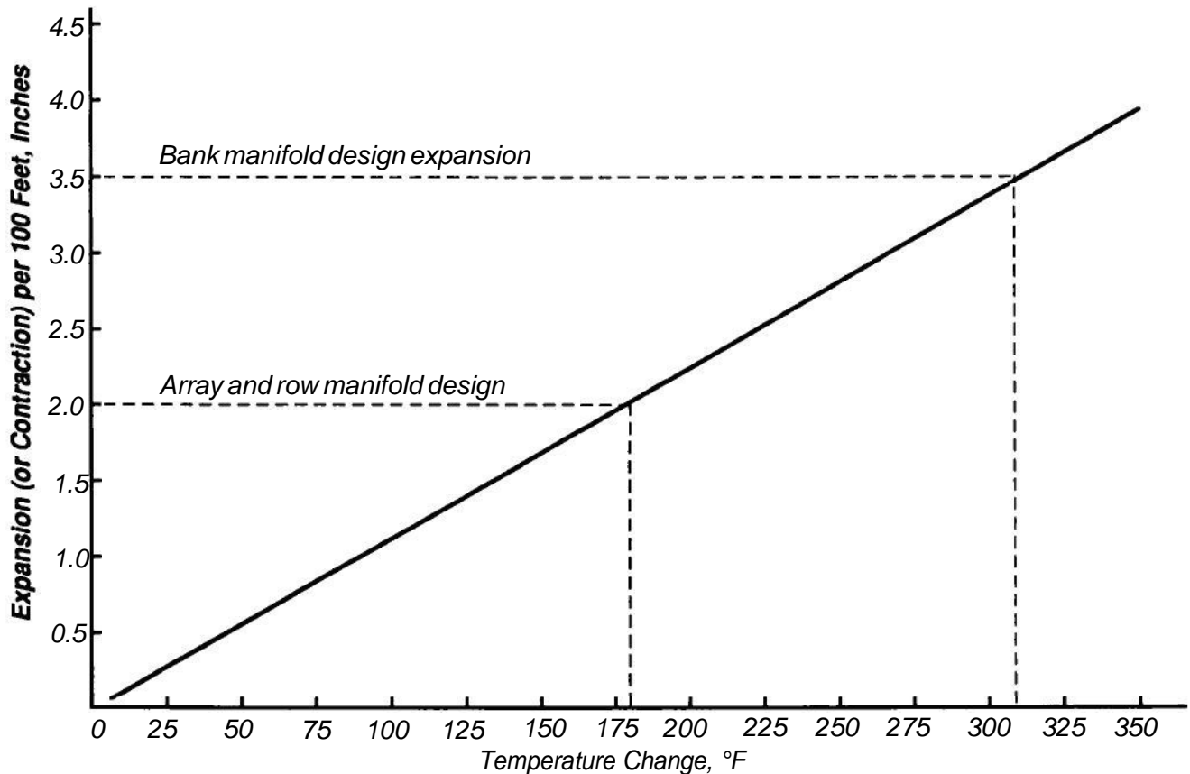
Figure 4-7. Thermal Expansion Versus Temperature Differential for Linear Copper Pipe.
