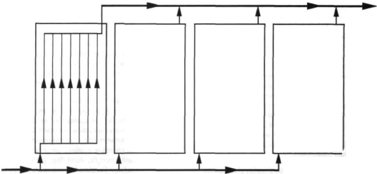
(b) Externally Manifoldeed Collectors
