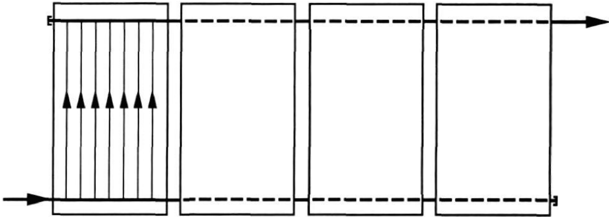
(a) Internally Manifoldeed Collectors (Required)
